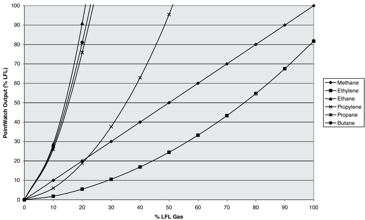
Methane Calibrated PointWatch - Response to Standard Gases
