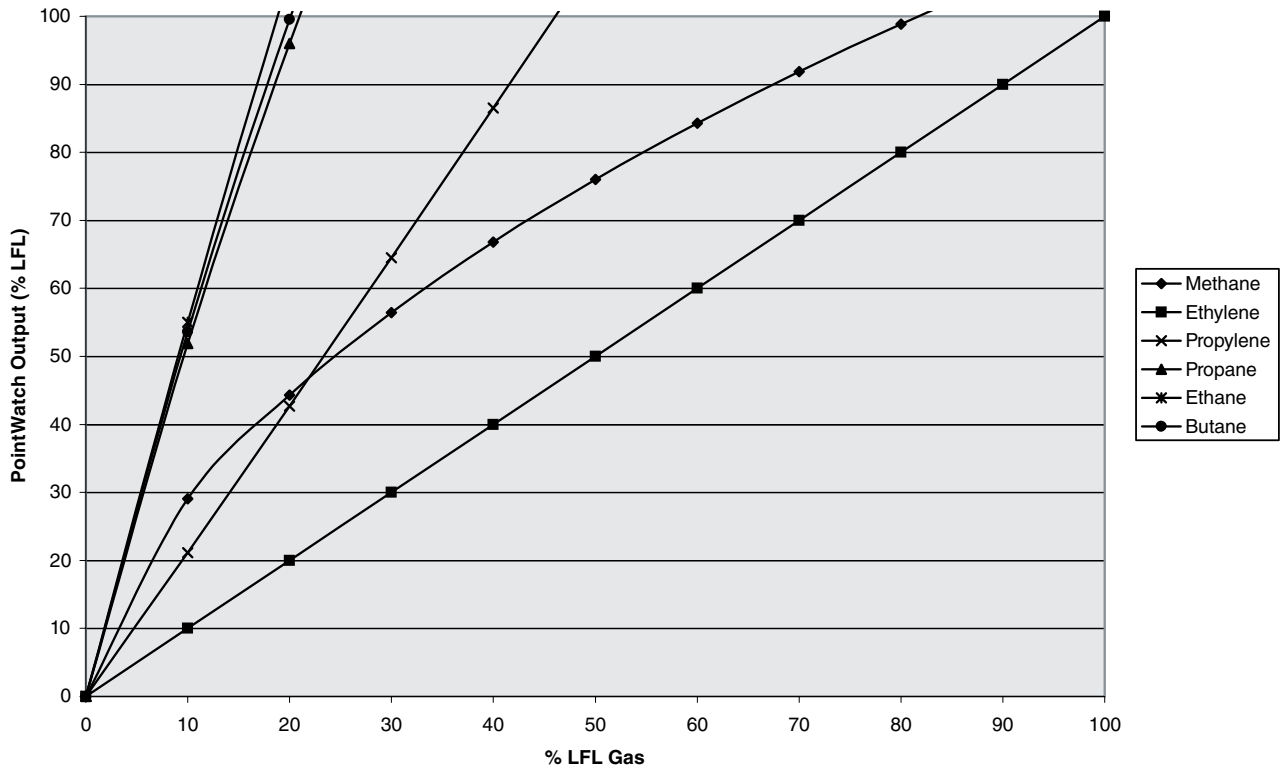
Ethylene Calibrated PointWatch - Response to Standard Gases
