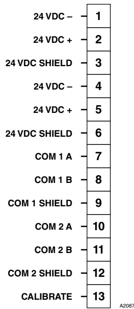
Figure 14—Wiring Terminal Identification for Eagle Quantum Premier Eclipse
