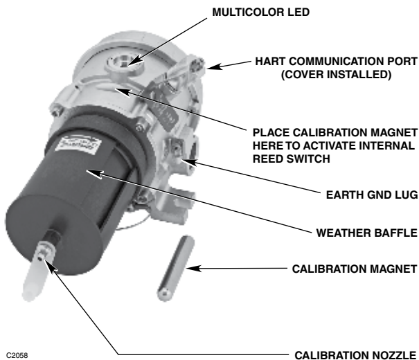
Figure 18—PointWatch Eclipse
