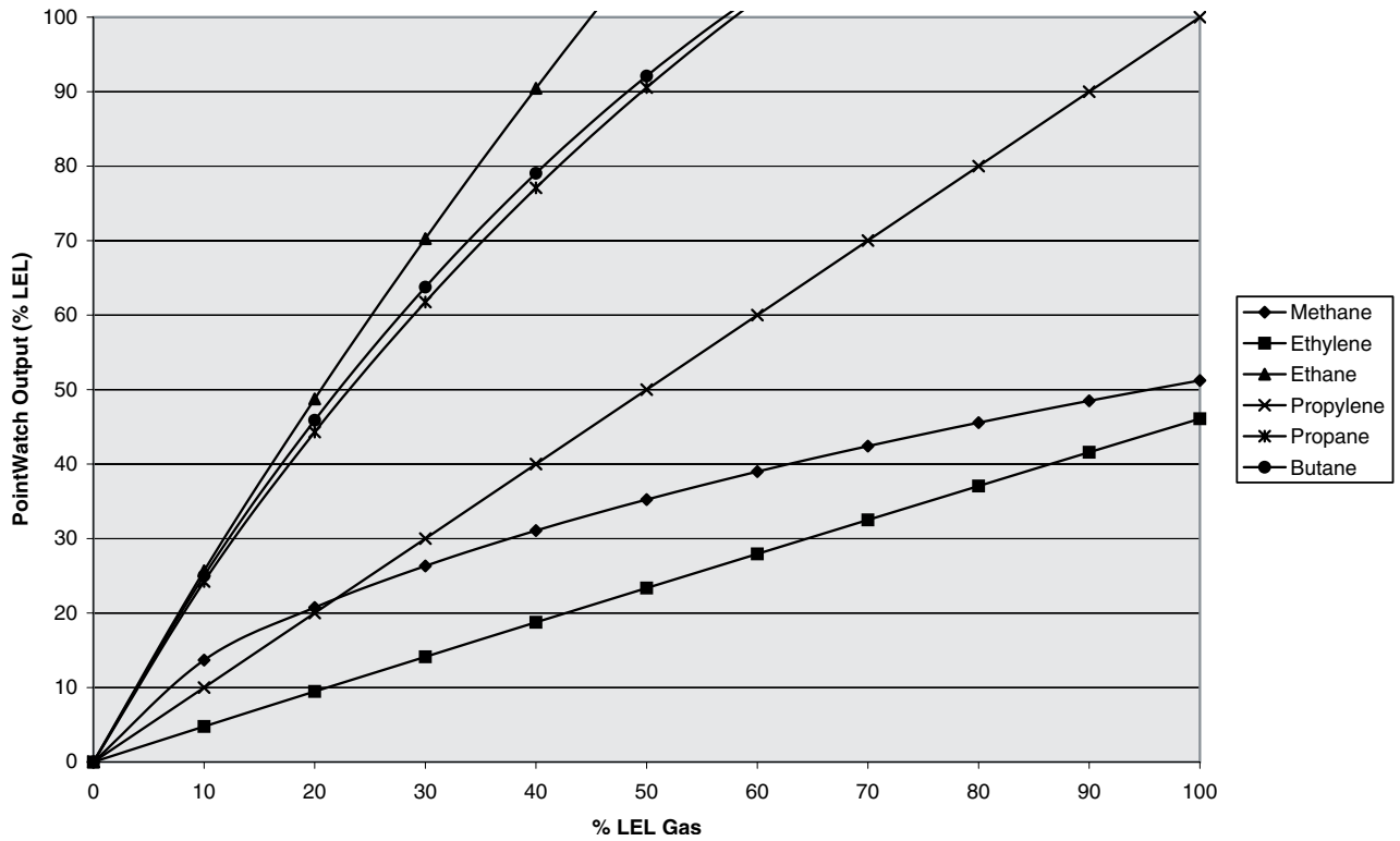
Propylene Calibrated PointWatch - Response to Standard Gases
